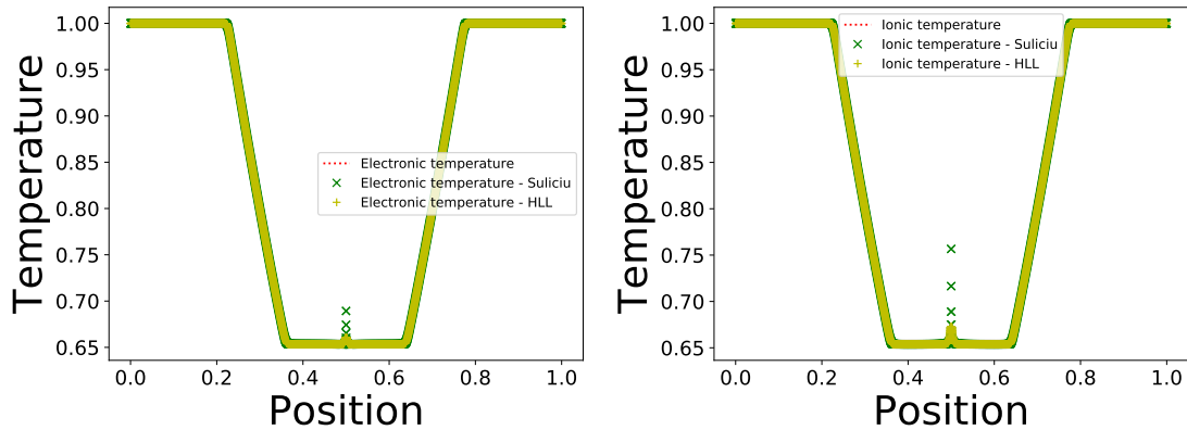
FIGURE 10. Temperature solutions of a rarefaction wave test case with a mass ratio of 10 with 120000 space points, 40 velocity points and a domain length of 8
