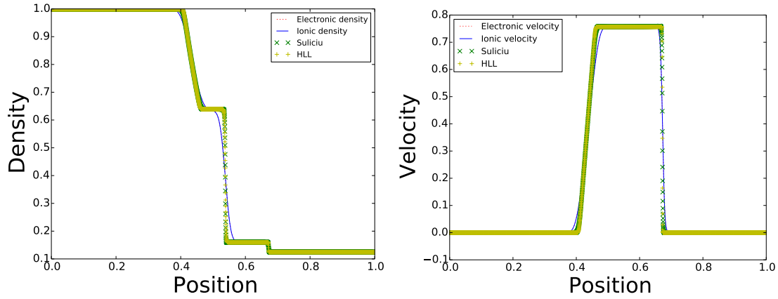
FIGURE 17. Density and velocity solutions of shock tube test case with a mass ratio of 1000 with 100000 space points, 40 velocity points and a domain length of 8
