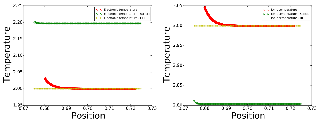
FIGURE 19. Different jump relations of electronic and ionic temperatures for a shock tube test case with a mass ratio of 1000 with 100000 space points, 40 velocity points and a domain length of 8
