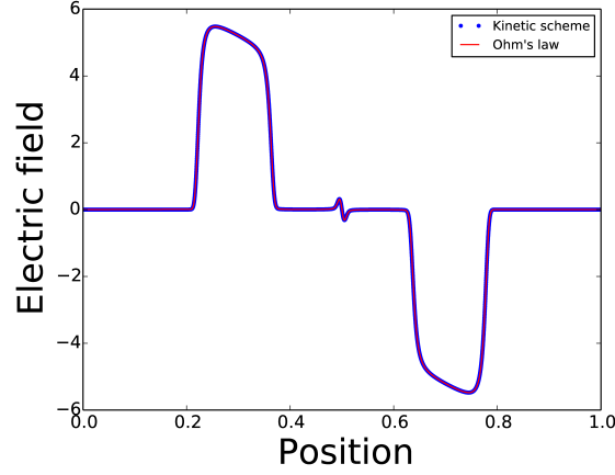
FIGURE 12. Electric field obtained by the kinetic scheme and by Ohm's law for the double rarefaction test case
