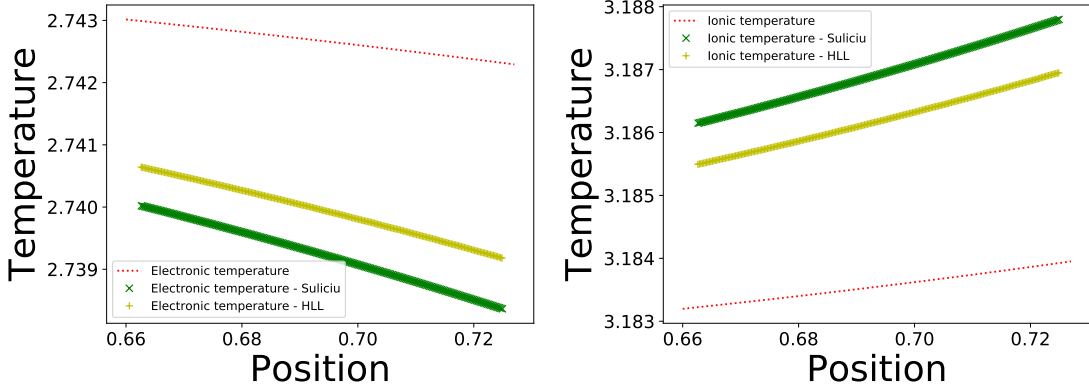
FIGURE 7. Different jump relations of electronic and ionic temperatures for a shock tube test case with a mass ratio of 10 with 120000 space points, 40 velocity points and a domain length of 8
