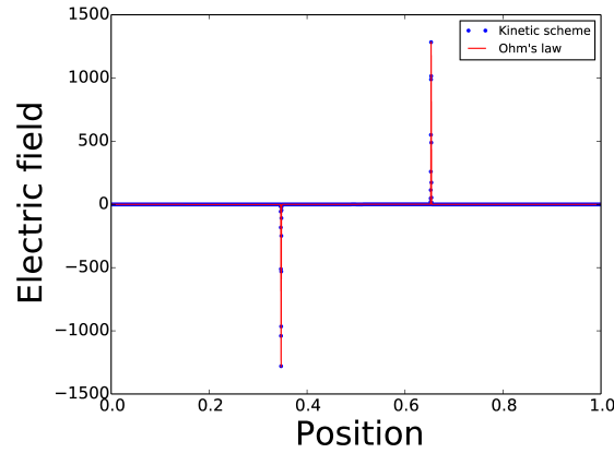
FIGURE 16. Electric field obtained by the kinetic scheme and by Ohm's law for the double shock test case
