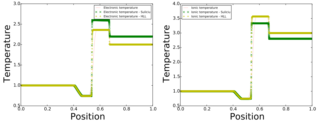
FIGURE 18. Electronic and ionic temperatures of a shock tube test case with a mass ratio of 1000 with 100000 space points, 40 velocity points and a domain length of 8
