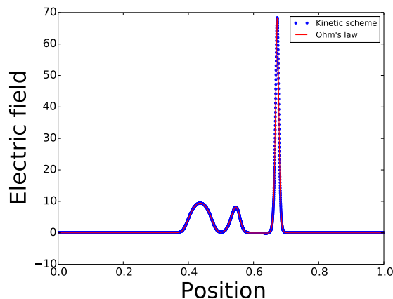
FIGURE 20. Electric field obtained by the kinetic scheme and by Ohm's law for a Sod tube test with different initial temperatures
