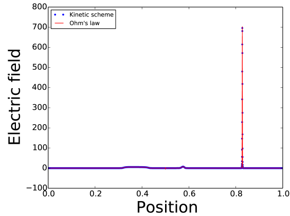
FIGURE 8. Electric field obtained by the kinetic scheme and by Ohm's law for the Sod tube test case with different initial temperatures
