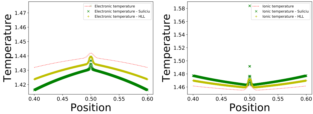
FIGURE 15. Electronic and ionic temperature of a shock wave test case with a mass ratio of 10 with 120000 space points, 40 velocity points and a domain length of 8
