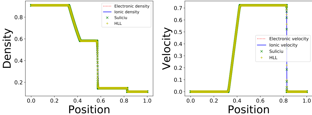
FIGURE 5. Density and velocity solutions of shock tube test case with a mass ratio of 10 with 120000 space points, 40 velocity points and a domain length of 8
