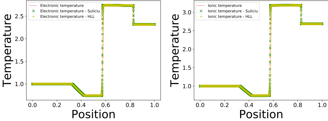
FIGURE 6. Electronic and ionic temperatures of a shock tube test case with a mass ratio of 10 with 120000 space points, 40 velocity points and a domain length of 8
