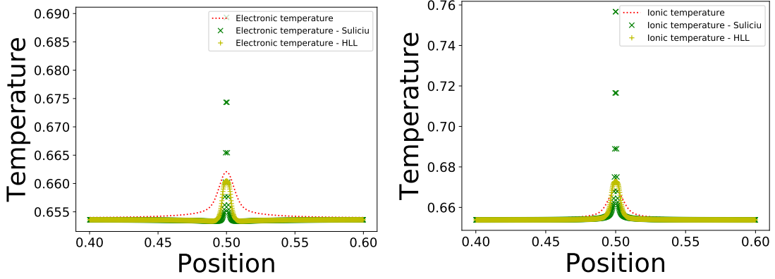
FIGURE 11. Zoom on temperature solutions of a rarefaction wave test case with a mass ratio of 10 with 120000 space points, 40 velocity points and a domain length of 8
