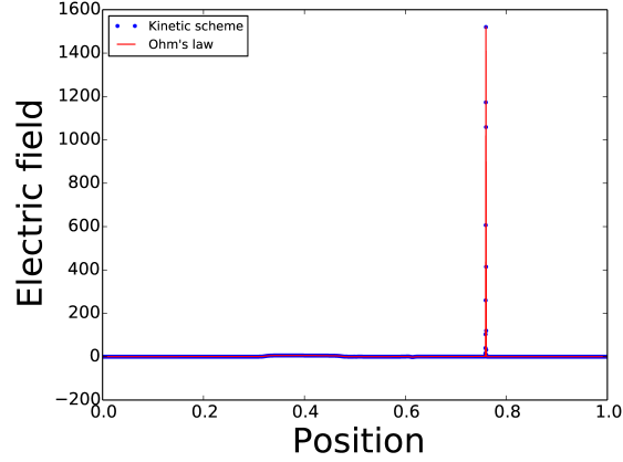
FIGURE 4. Electric field obtained by the kinetic scheme and by Ohm's law for the Sod tube test case with identical initial temperatures
