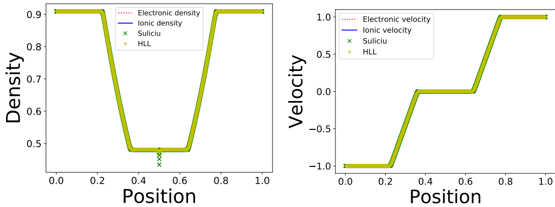
FIGURE 9. Density and velocity solution of a rarefaction wave test case with a mass ratio of 10 with 120000 space points, 40 velocity points and a domain length of 8
